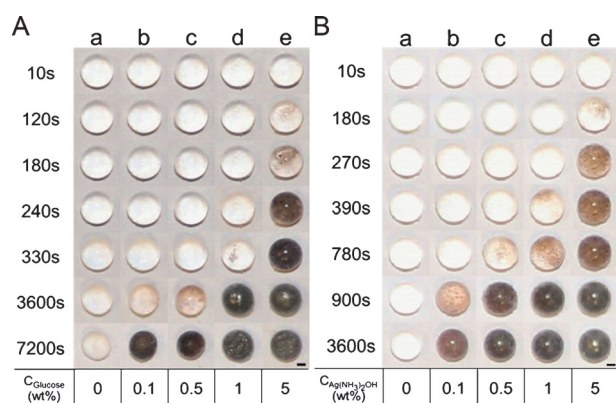
Figure 2. Photographic images of liquid marbles with various diamminesilver(I) and glucose concentrations captured at different reaction stages: A) liquid marbles with fixed diamminesilver(I) concentration (5 wt%) and increasing glucose concentrations. a) 0, b) 0.1, c) 0.5, d) 1, and e) 5 wt%; B) liquid marbles with fixed glucose concentration (5 wt%) and increasing diamminesilver(I) concentrations. a) 0, b) 0.1, c) 0.5, d) 1, and e) 5 wt%. Scale bars: 1 mm.
